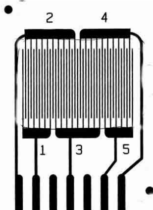
Test Coupon: "Typical Comb Pattern" (JIS C 6480 coupon)
